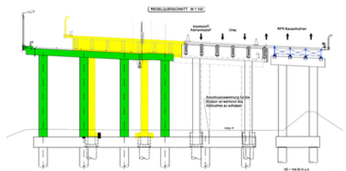
Overview of the phased construction. Source: PORR
